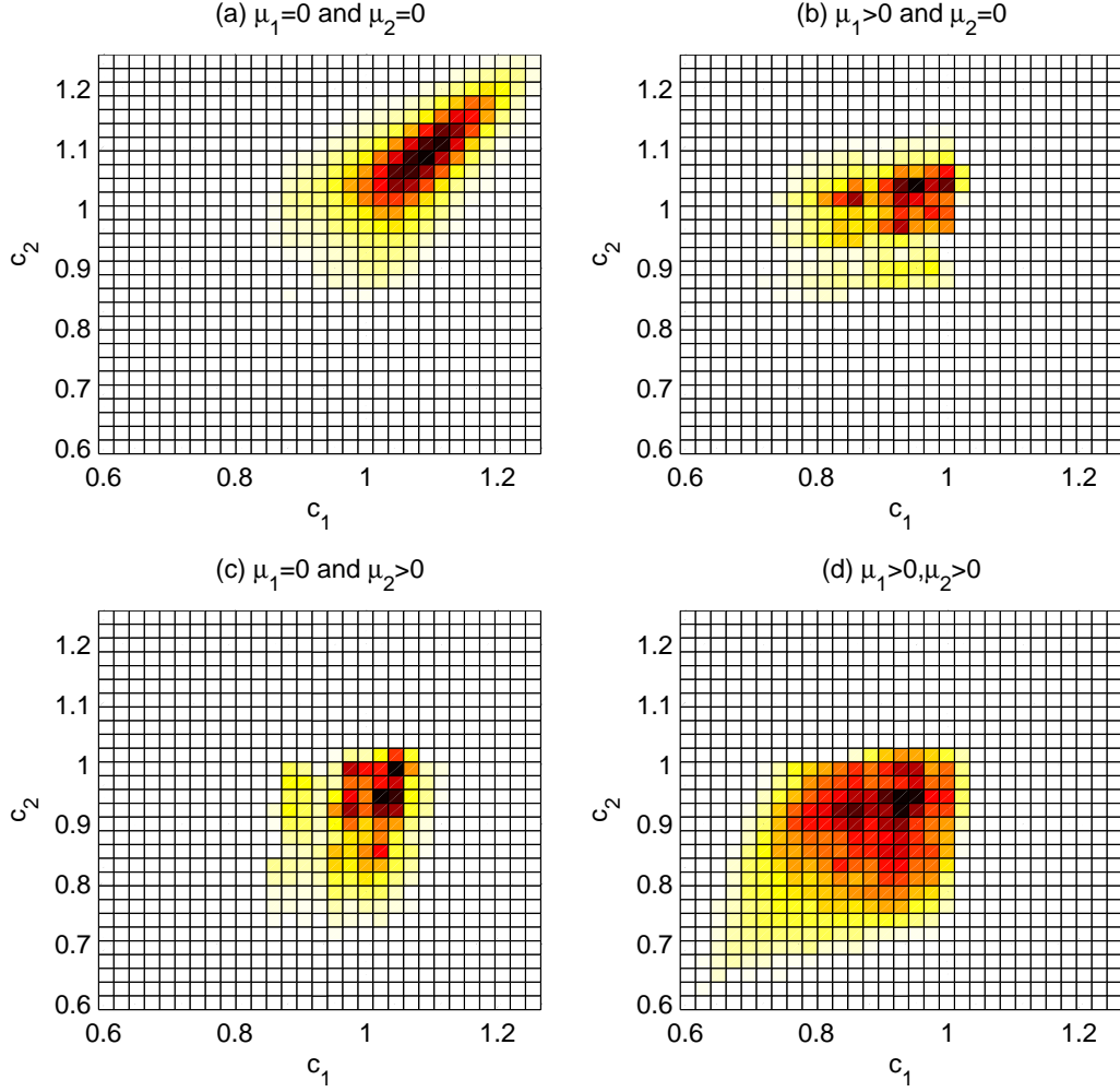
Figure 7: Investors' consumption distribution along a simulated path of 200,000 periods in bond market integration. The darker an area is, the higher the frequency becomes. Panel (a) displays the distribution of consumption when investors in both countries are financially unconstrained, panel (b) for only investors in country 1 constrained, panel (c) for only investors in country 2 constrained, and , panel (d) for investors in both countries constrained. Model parameters are the same as the baseline model.
